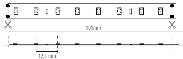
LED SPACING AND PITCH CUT 8 LED (7,2W)
