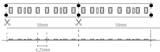
LED SPACING AND PITCH CUT 8 LED (14,4W)
